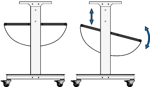
Catch is adjustable vertically and horizontally
